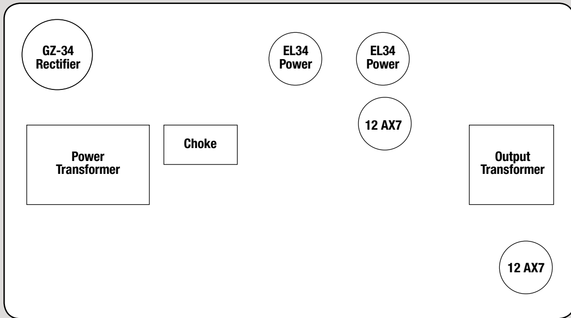
FRONT PANEL
