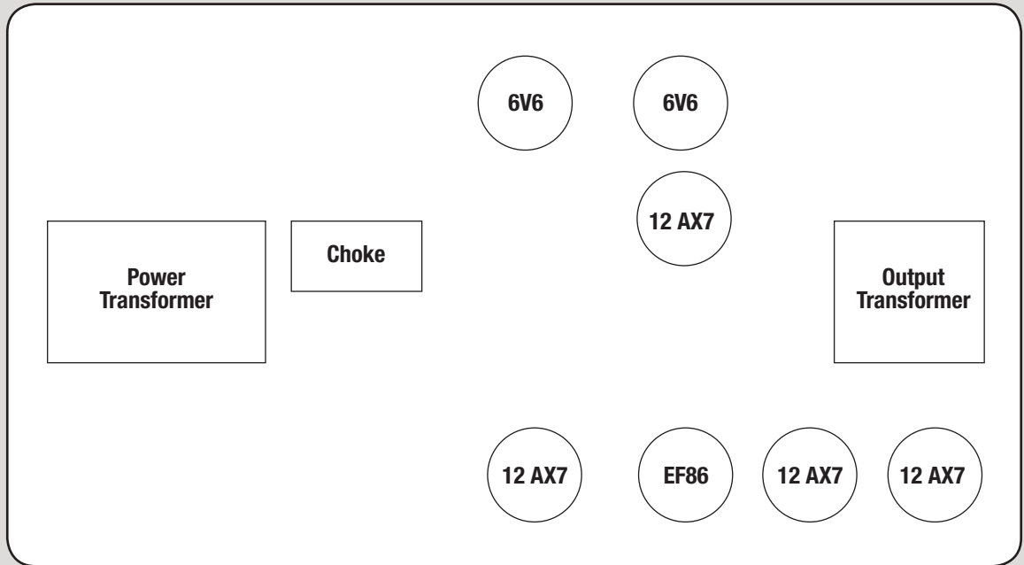
FRONT PANEL
